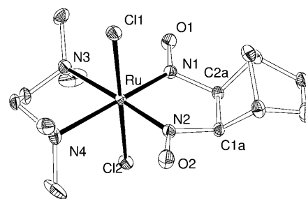
Figure 2. ORTEP representation of 4a ; thermal ellipsoids at 20% probability. Selected bond angles [°] and lengths [Å]: N1–Ru 1.879(3), N2–Ru 1.883(3), N3–Ru 2.259(4), N4–Ru 2.266(3), Cl1–Ru 2.3706(12), Cl2–Ru 2.3930(16), N1–O1 1.231(4), N2–O2 1.227(4), N1–C2A 1.508(3), N2–C1A 1.524(3), C1A–C2A 1.5448(4); N2–Ru–N1 84.33(14), N3–Ru–N4 81.32(14).
