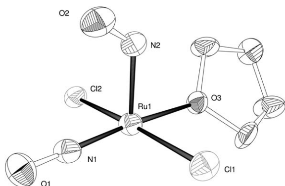
Figure 1. ORTEP representation of 2 ; thermal ellipsoids at 50% probability. Selected bond angles [°] and lengths [Å]: Ru–N1 1.727(5), Ru–N2 1.915(5), Ru–O3 2.110(4), Ru–Cl1 2.349(2), Ru–Cl2 2.392(2), N1–O1 1.147(6), N2–O2 1.181(6); O1–N1–Ru 178.5(6), O2–N2–Ru 124.0(4).
